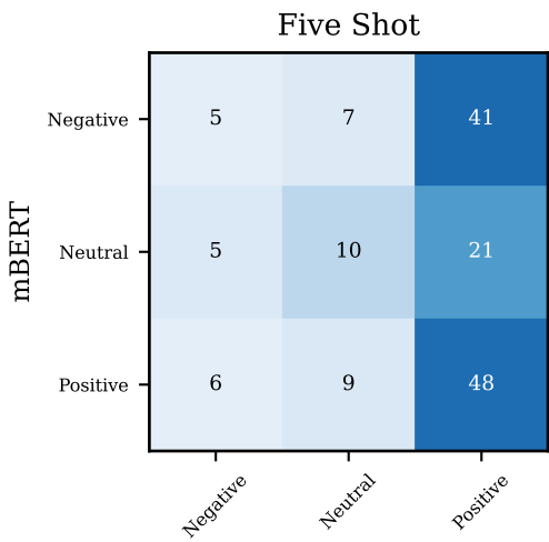
Confusion Matrices: Every Model x Every Learning Setting (SentMix-3L, counts shown, color = row-normalized)
