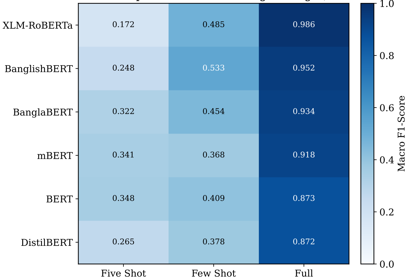
Macro-F1 Heatmap: Models vs. Learning Settings (SentMix-3L)
