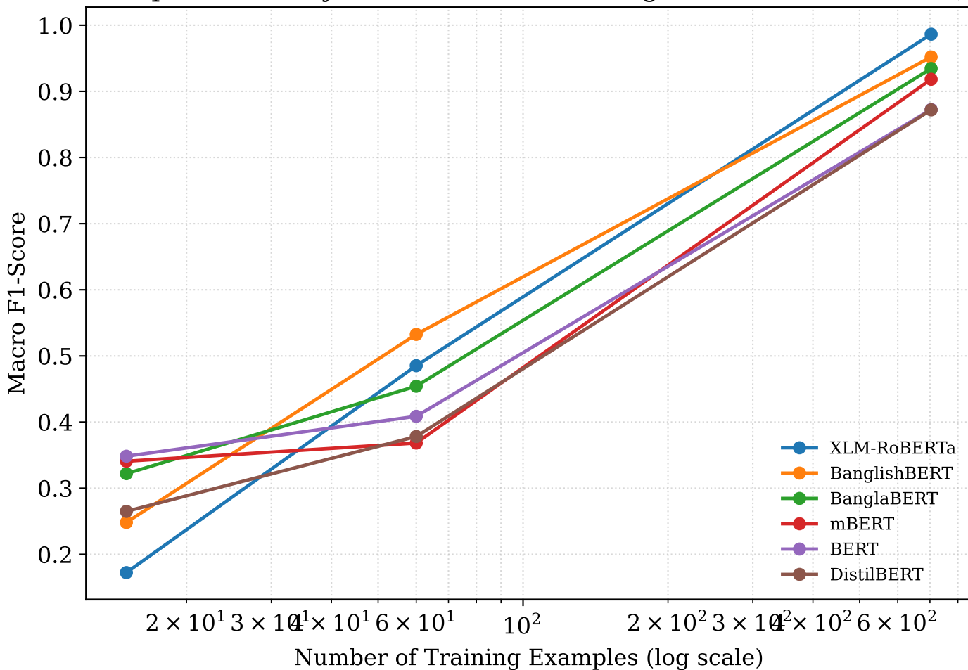
Sample Efficiency: Macro-F1 vs. Training Set Size (SentMix-3L)
