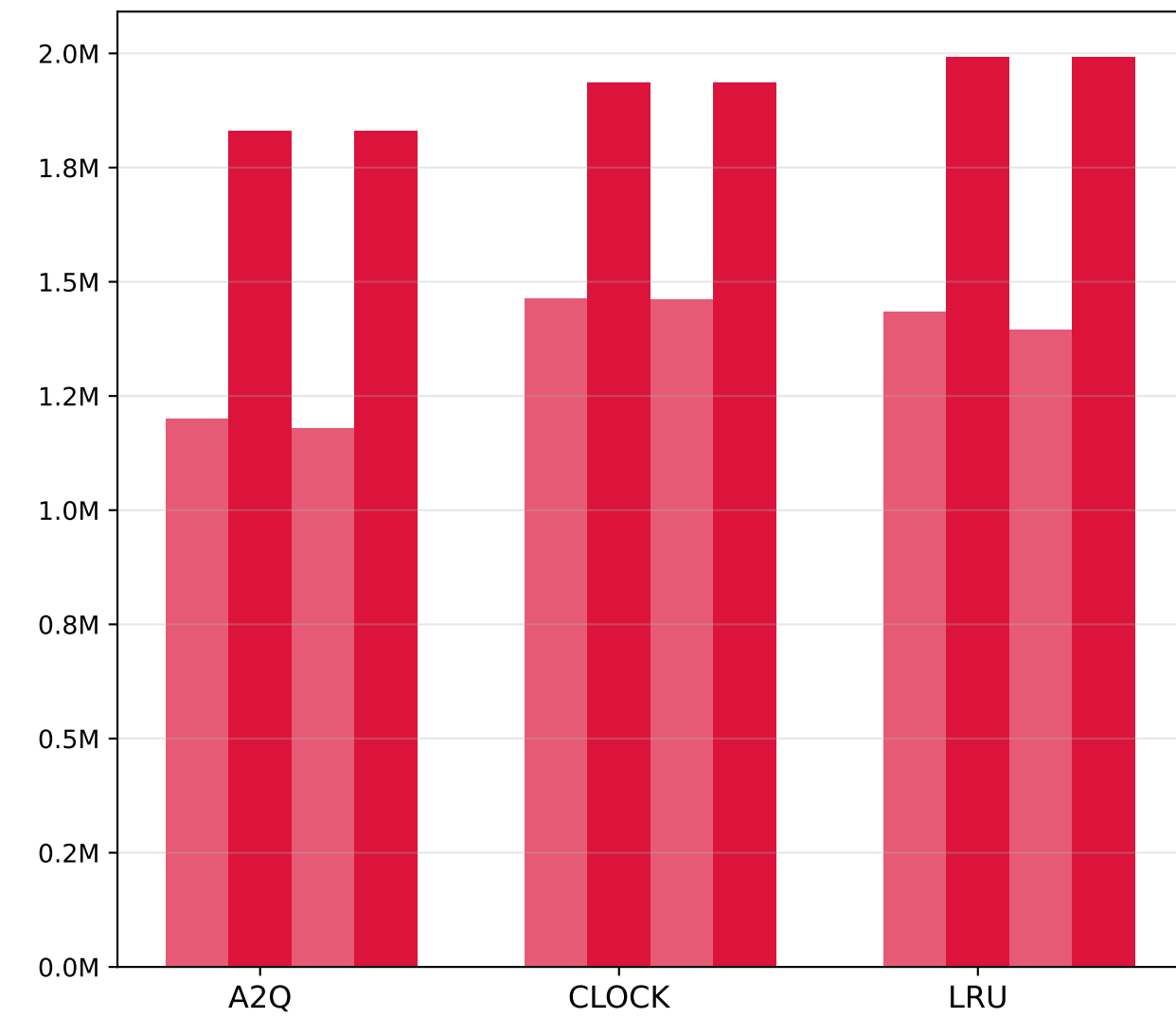
SSD NVMe - Cache Misses
