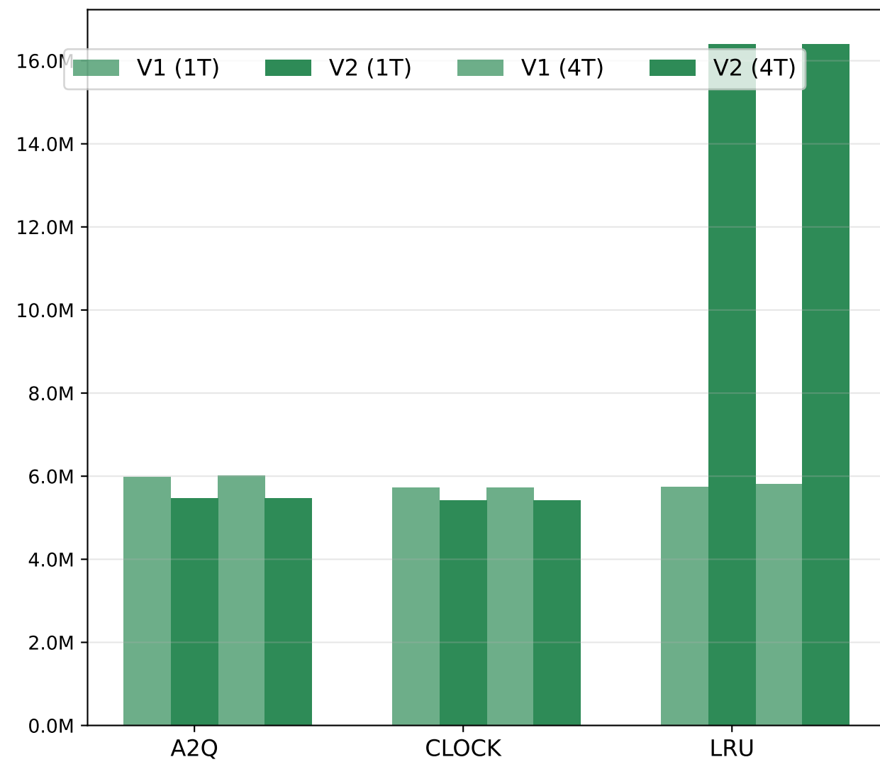
NVM - Cache Misses
