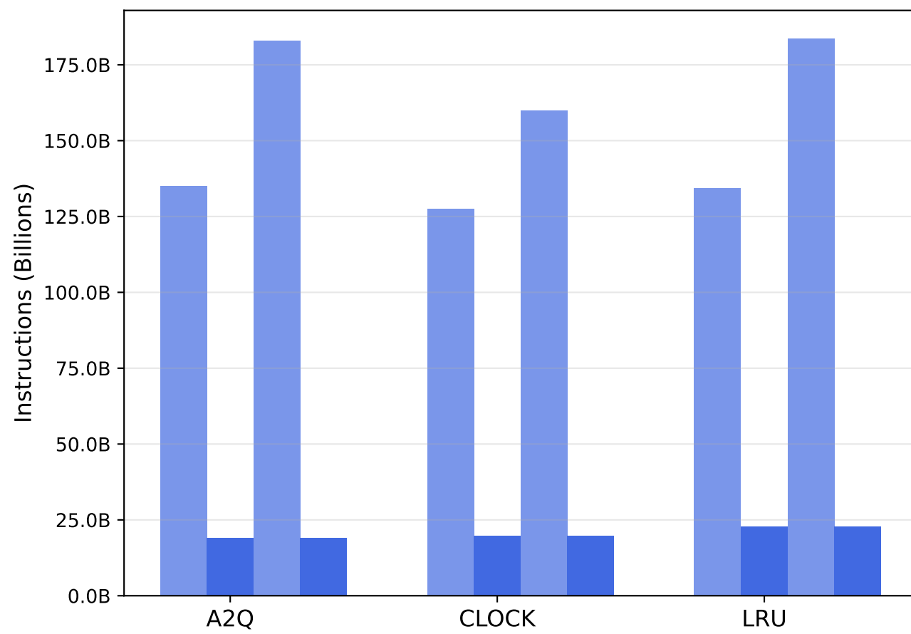
NVDIMM - User Time
