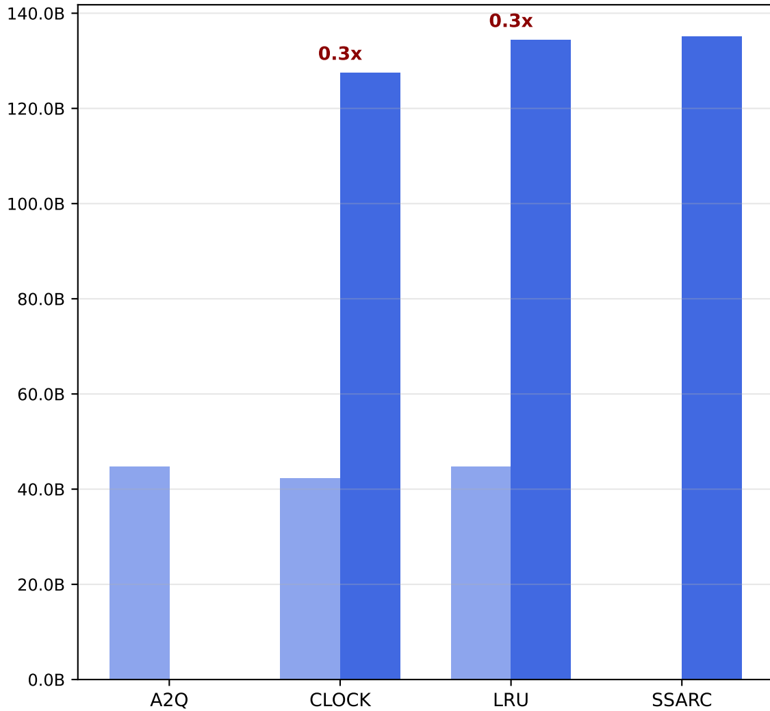
Throughput
