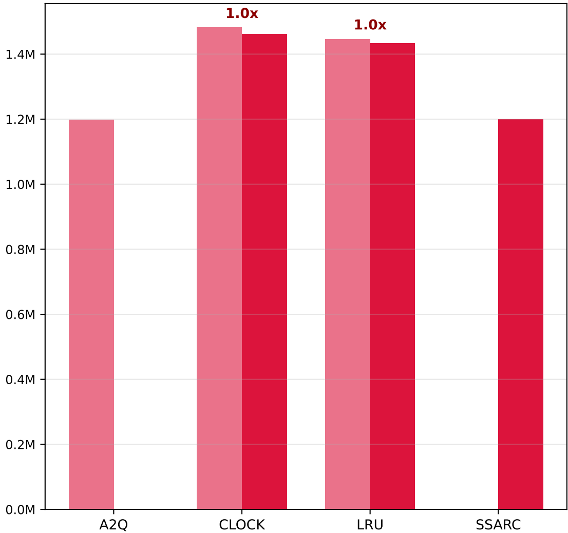
System Time
