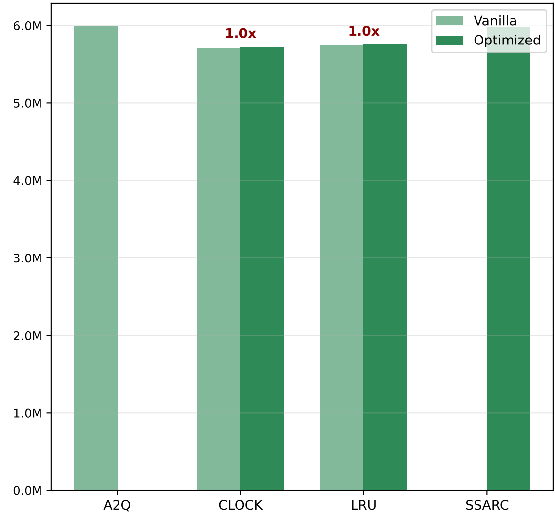
User Time
