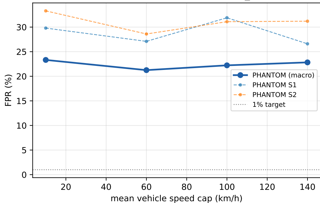
(b) False-positive rate vs speed ( \alpha_v test)
