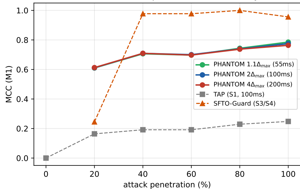
(a) Detection vs penetration & intensity
