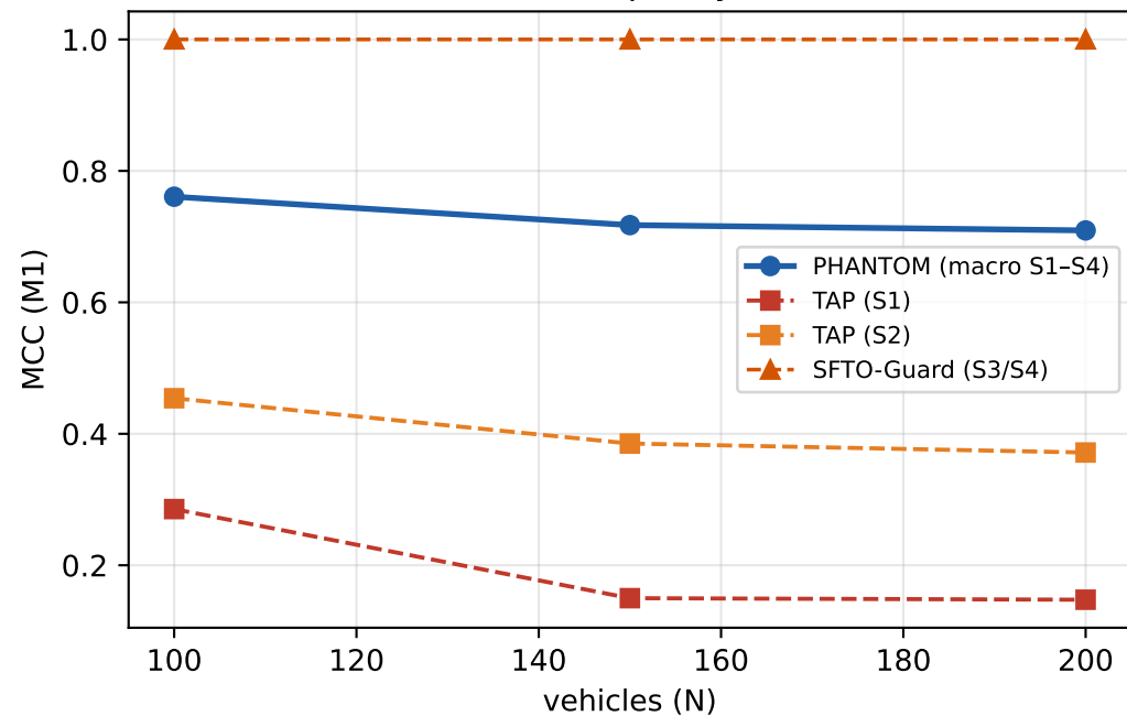
(a) Detection quality vs scale
