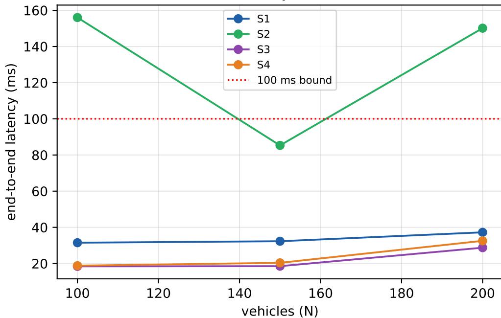
(b) Latency vs scale
