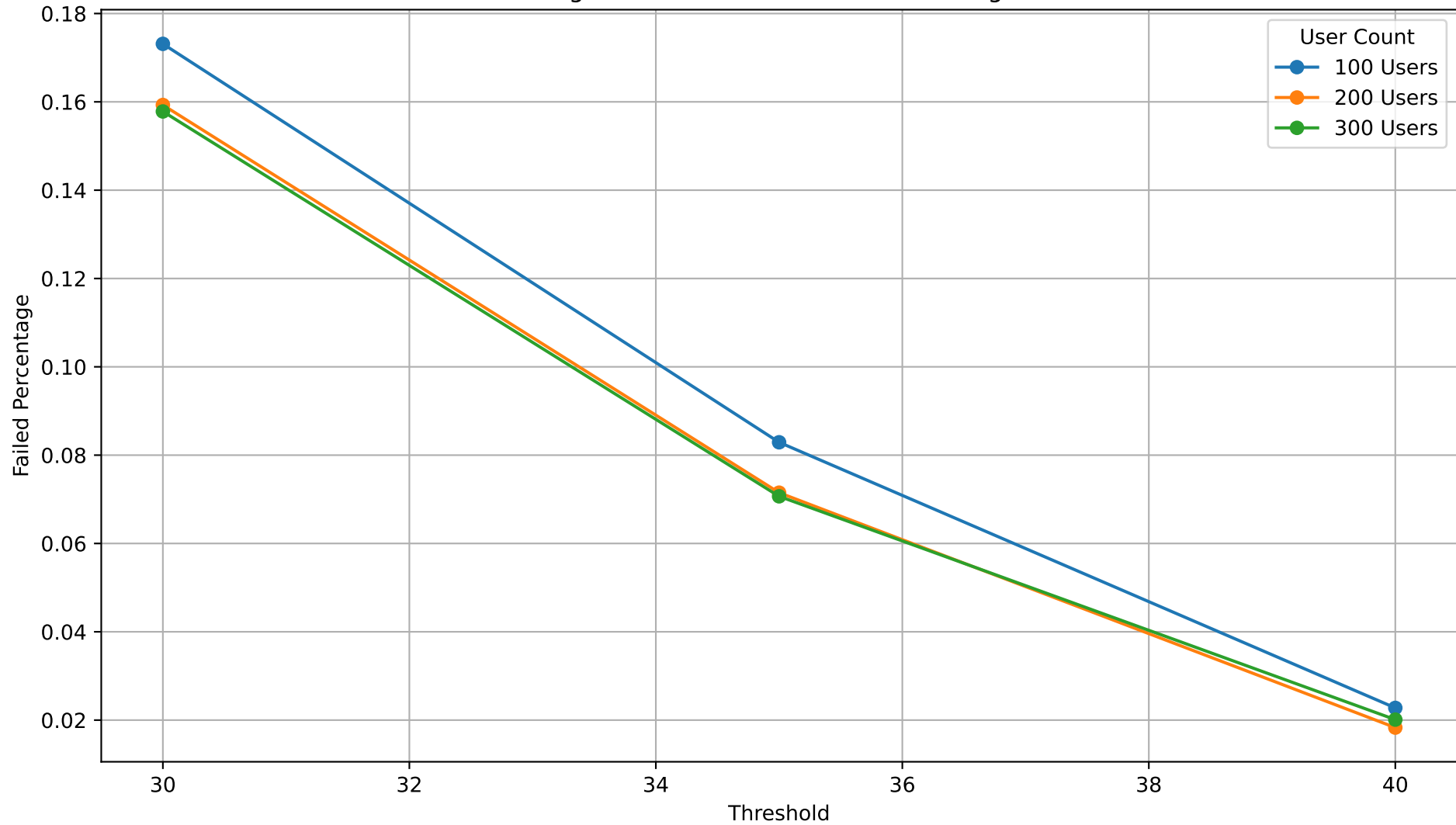
Failed Percentage vs Threshold for Different Benign User Counts
