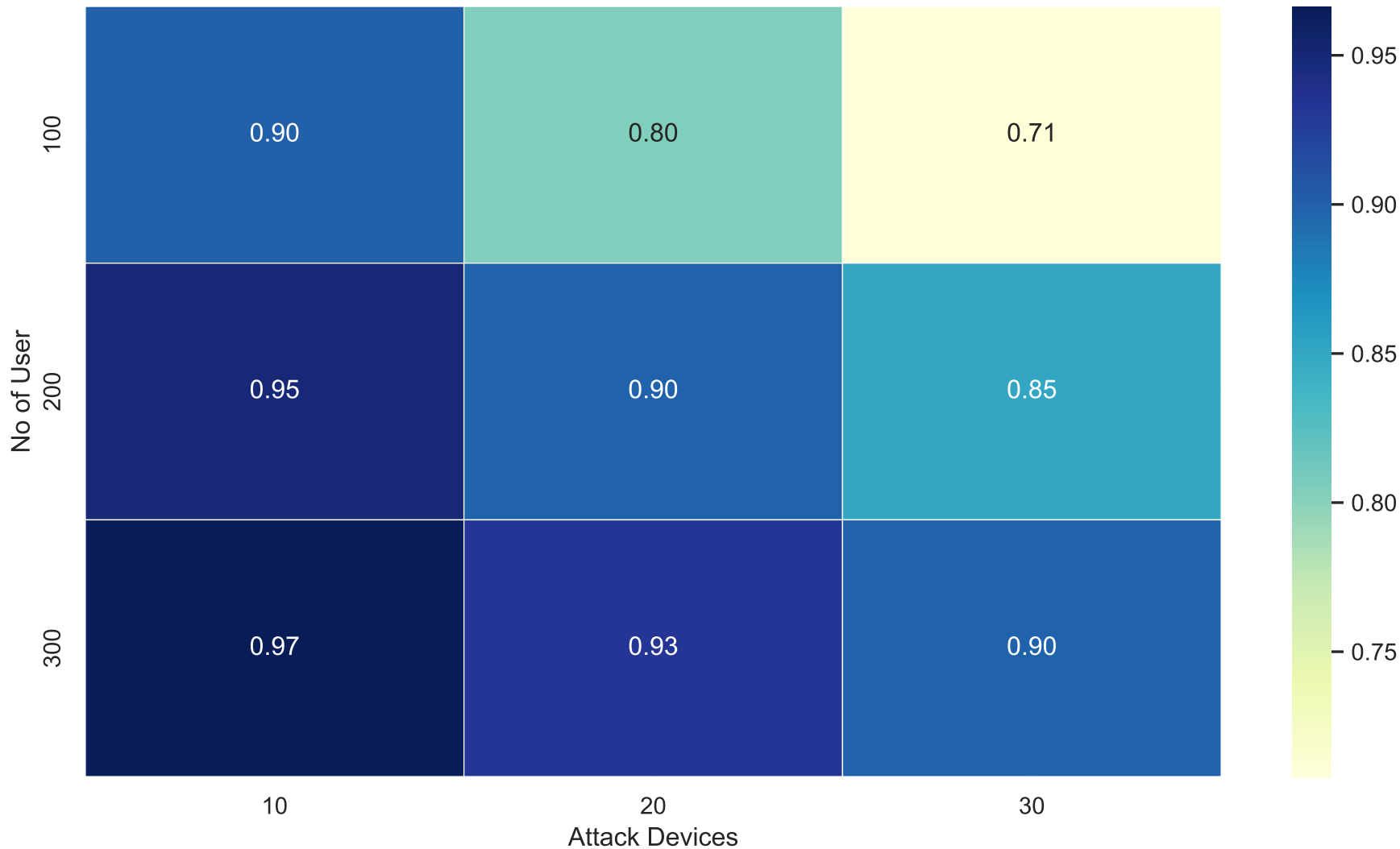
Failed Percentage Heatmap (No of User vs Attack Devices)
