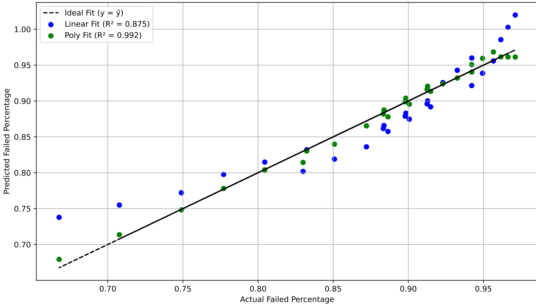
Actual vs Predicted Failed Percentage
