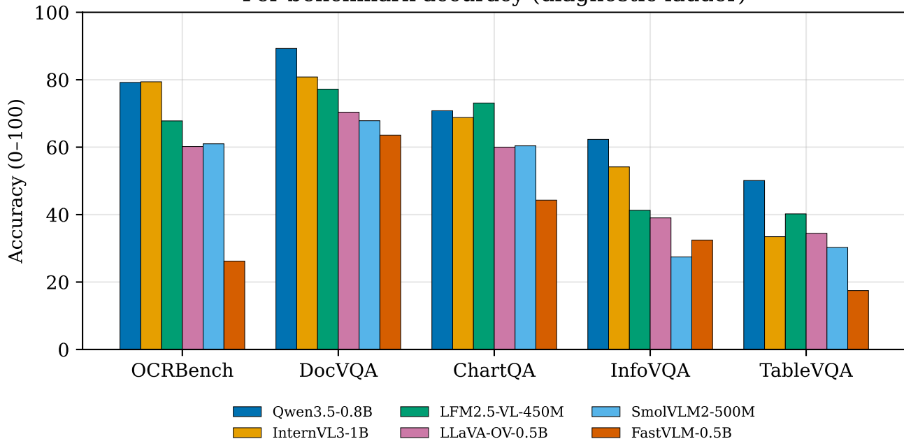
Per-benchmark accuracy (diagnostic ladder)
