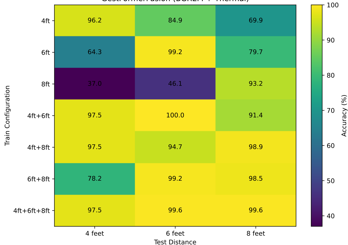
Cross-Distance Accuracy Heatmap GestFormerFusion (BGREM + Thermal)
