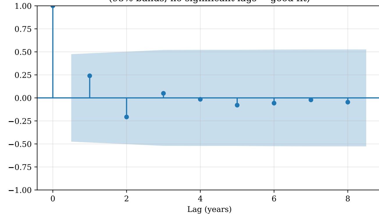
Panel C: ACF of score residuals (95% bands; no significant lags = good fit)
