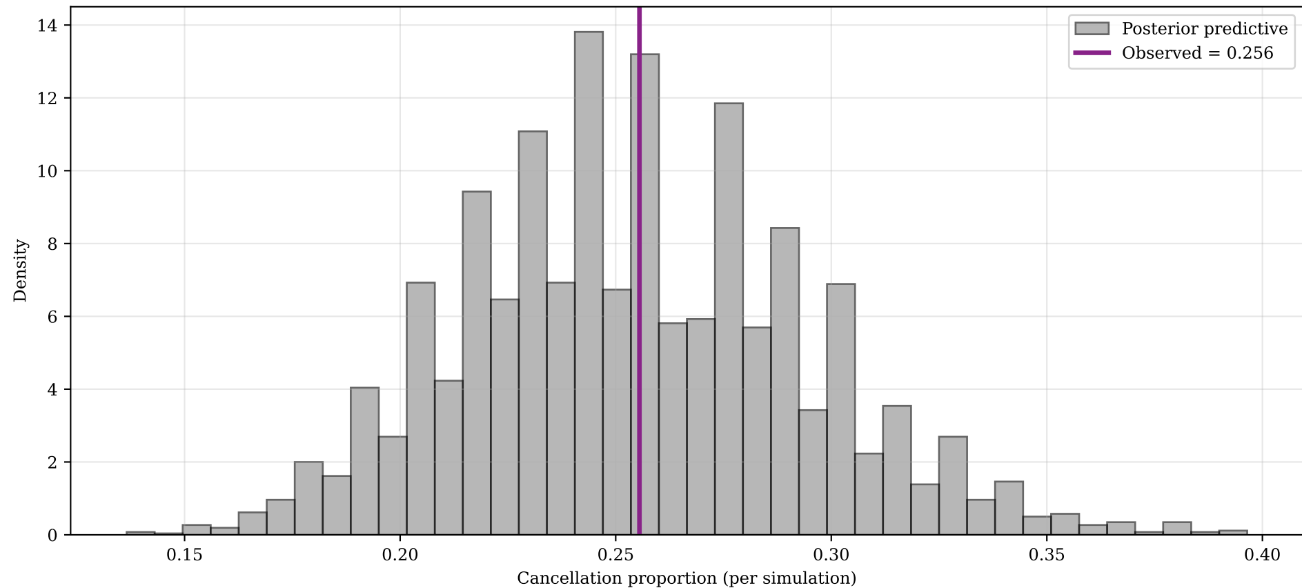
Figure: Posterior predictive check — overall cancellation rate PPC p=0.492 (acceptable 0.05 < p < 0.95 )
