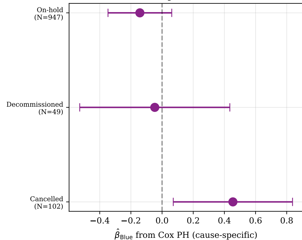
Panel C: S&P — Blue HR per outcome (cause-specific Cox PH)
