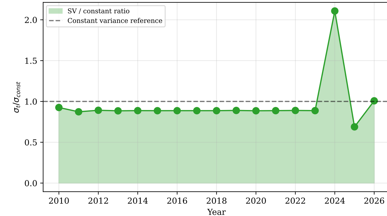
Panel C: Volatility ratio over time ( >1 = above constant-var level)
