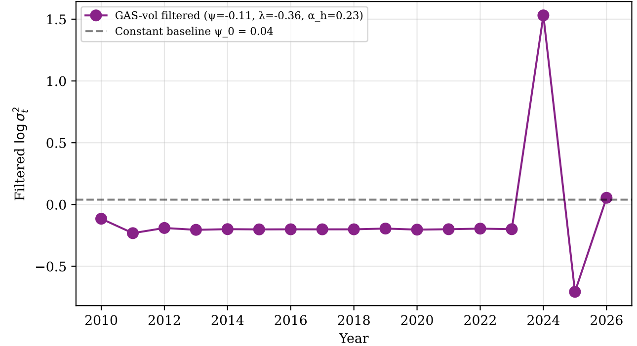
Panel B: Filtered log-variance path LR = 2.46, p = 0.292
