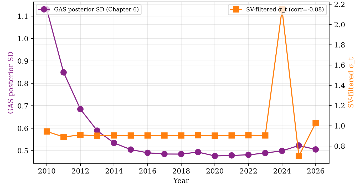
Panel D: GAS uncertainty vs SV vol (corr = -0.081)
