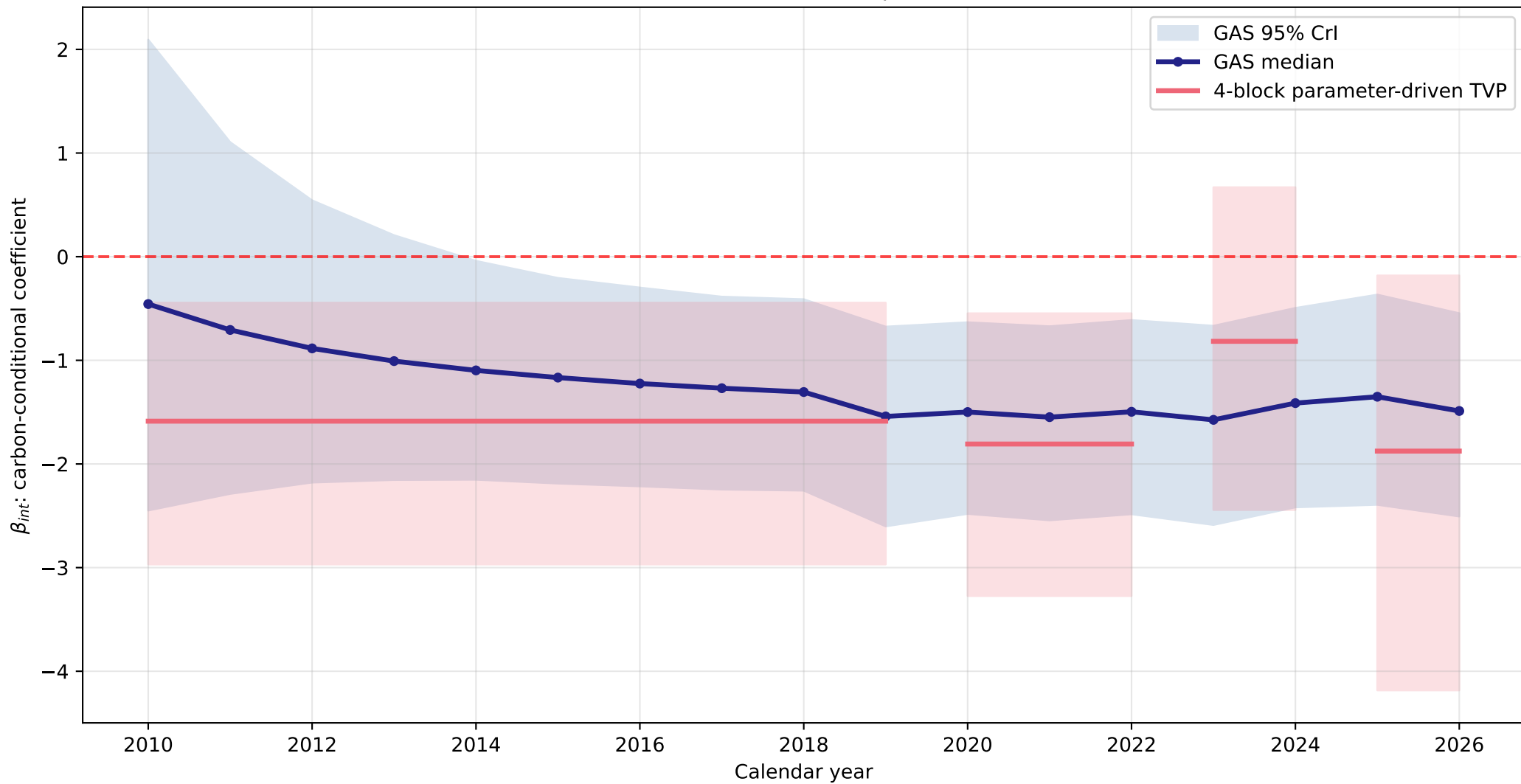
GAS observation-driven vs 4-block parameter-driven TVP
