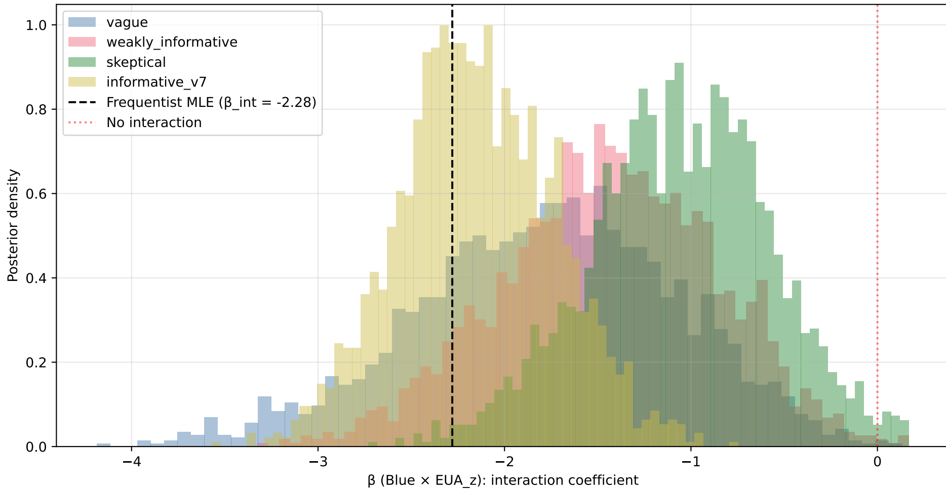
Posterior of carbon-conditional interaction coefficient across priors
