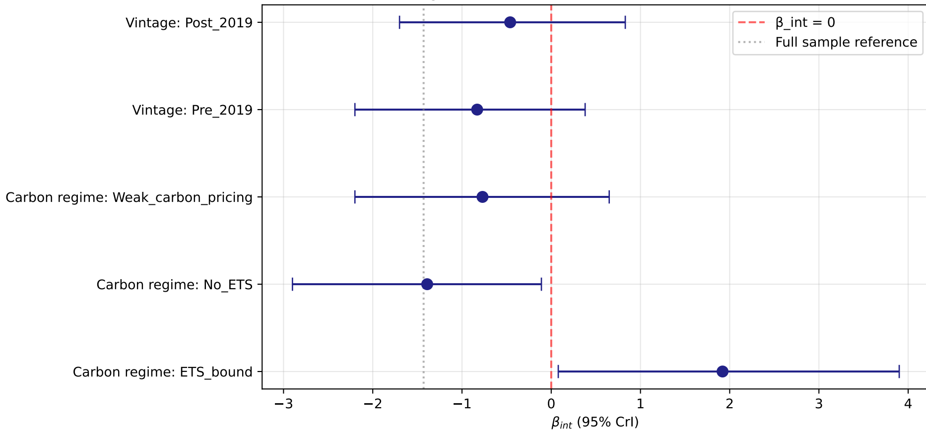
Heterogeneous carbon-conditional effects across strata
