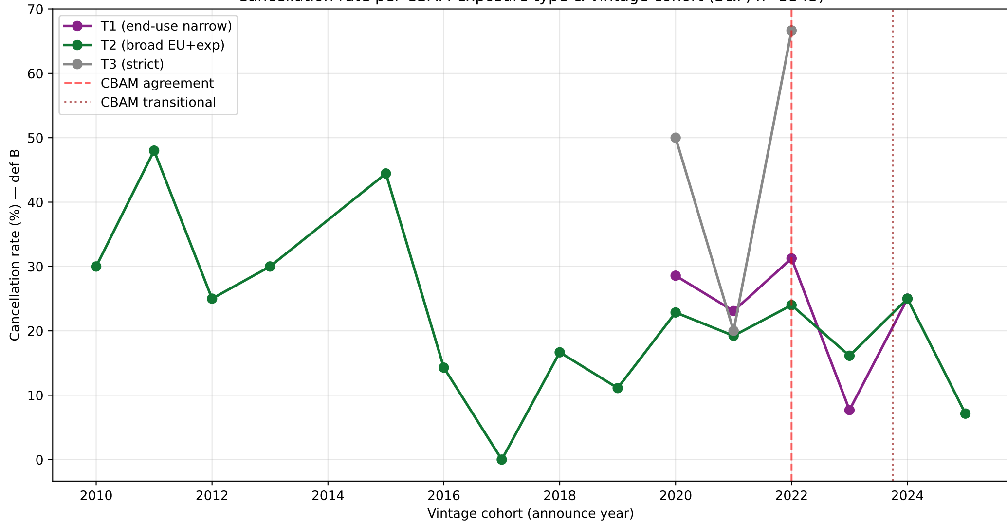
Cancellation rate per CBAM exposure type & vintage cohort (S&P, n=3343)
