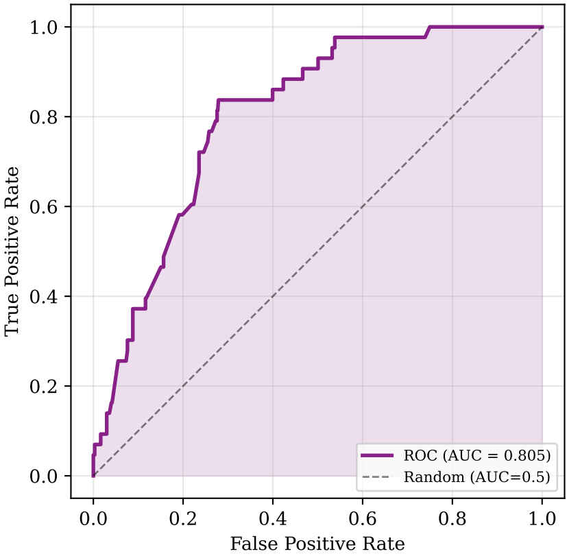
Panel A: ROC curve
