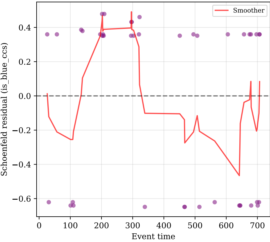
Panel E: Schoenfeld residuals is_blue_ccs PH test p=0.374
