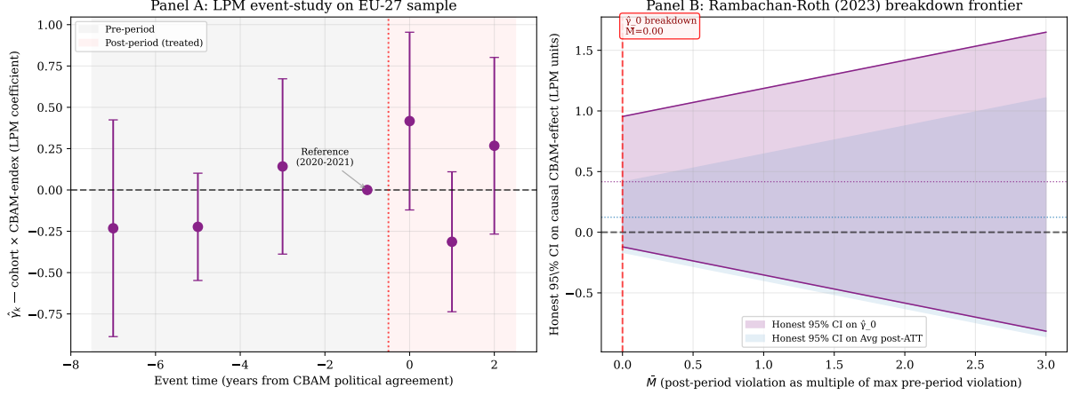
Figure 5: Honest DiD analysis of EU-only event-study. Panel A: event-time \times CBAM-index coefficients (LPM) with 95% CIs. Pre-treatment coefficients (gray-shaded region) provide evidence of parallel-trends violations. Panel B: Rambachan-Roth (2023) breakdown frontier under the relative-magnitudes restriction \Delta^{\text{RM}}(\bar{M}) . Purple shading shows Honest 95% CI on the focal ATT ( \hat{\gamma}_0 ); blue shading shows the same for the average post-period ATT. The breakdown \bar{M} = 0.00 indicates that zero enters the CI under the strictest possible relaxation (no post-period violations), demonstrating that the cross-sectional EU pattern is not identifiable as a causal CBAM effect.
