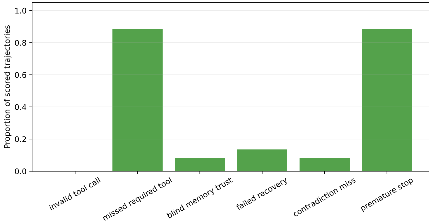
Failure mode distribution
