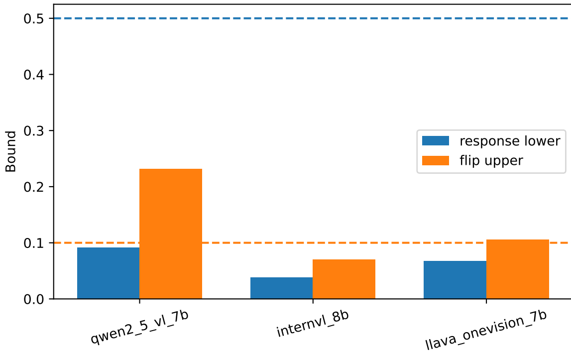
Historical exact certificate bounds
