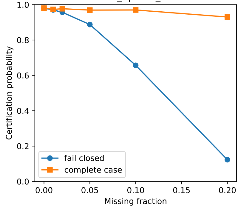
semantic_update_success
