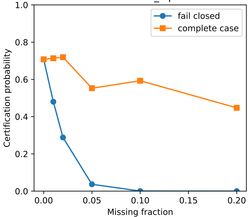
irrelevant_flip
