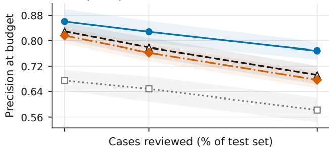
(a) Elliptic / precision
