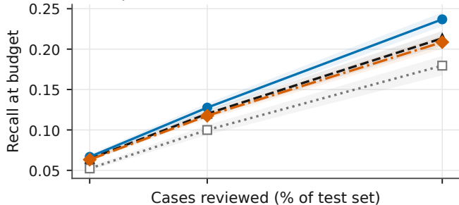
(b) Elliptic / recall
