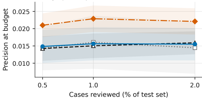
(c) Dgraphfin / precision
