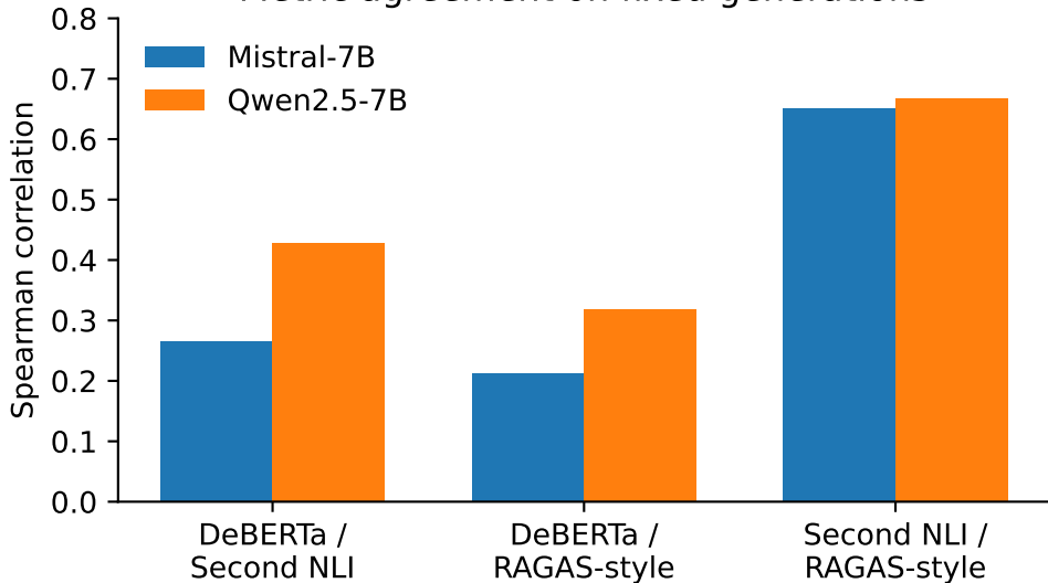
Metric agreement on fixed generations
