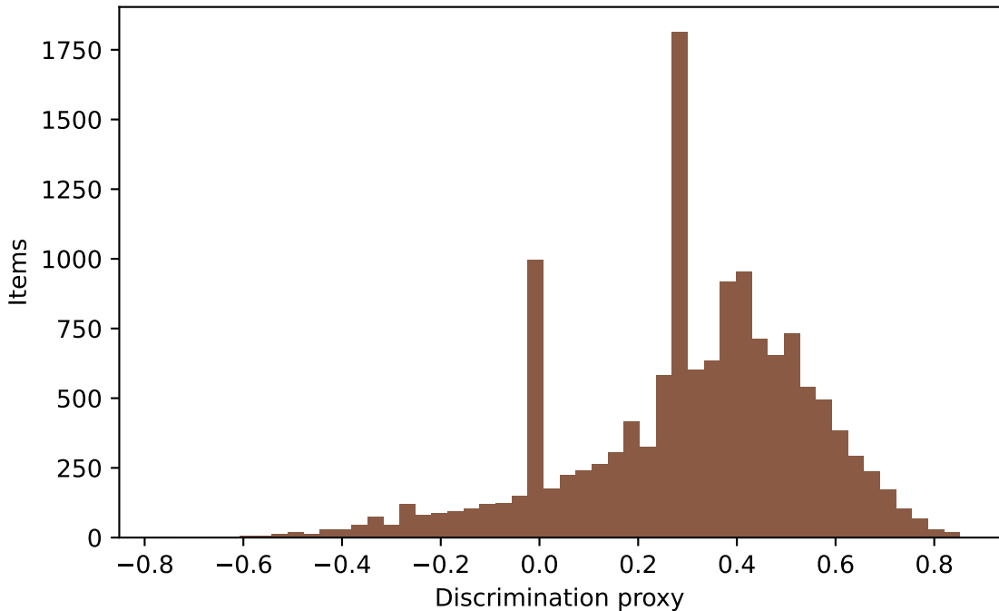
MMLU discrimination distribution
