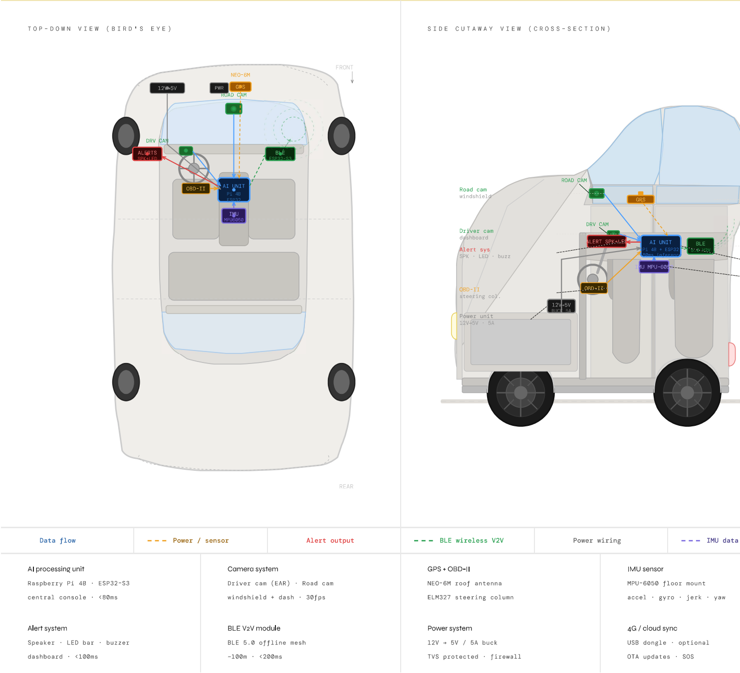
PROJECT GARUDA · VEHICLE INSTALLATION BLUEPRINT · DUAL VIEW Top-down + Side cutaway · Real hardware placement · Edge AI · BI
