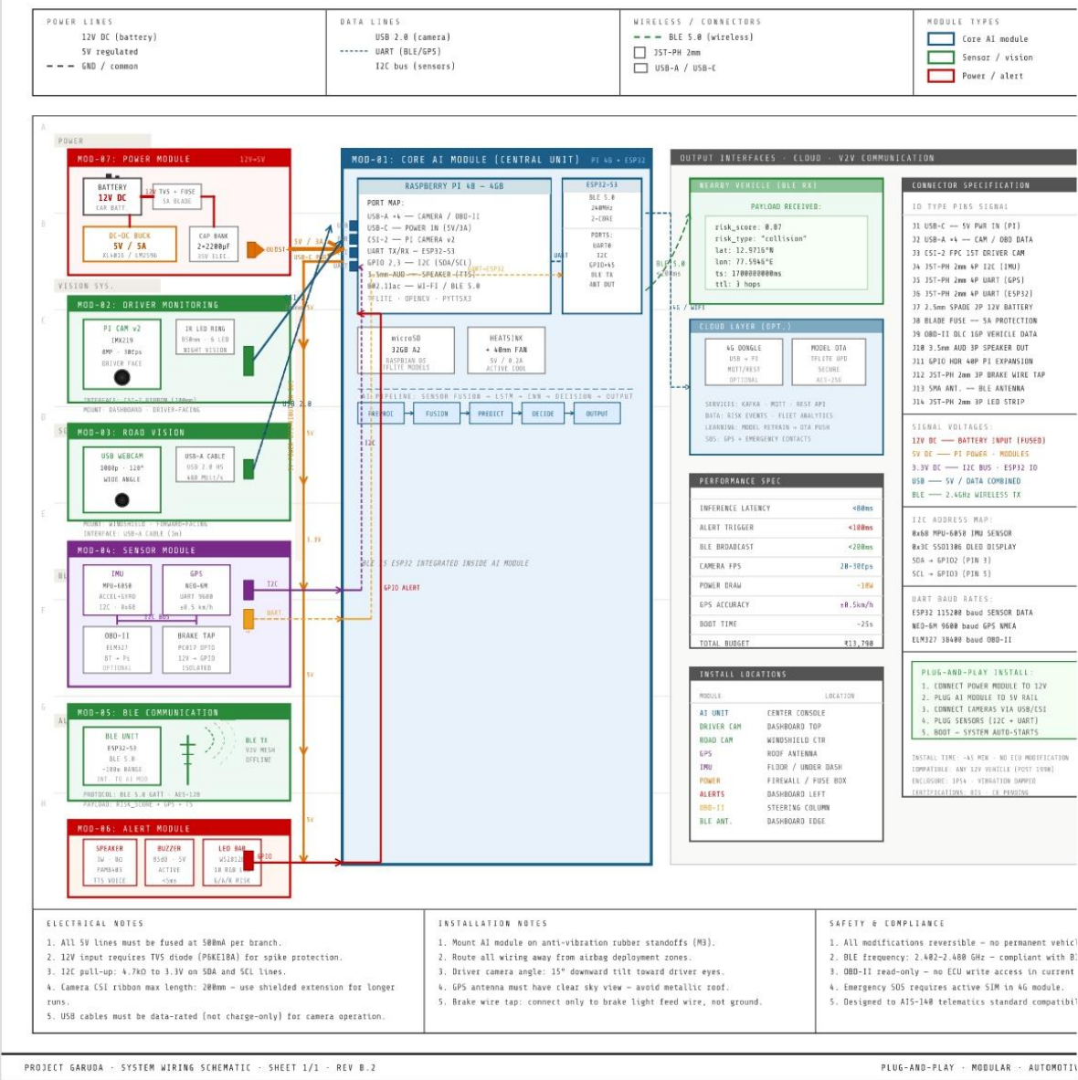
(Fig 1.5 – Auto Cad Diagram)
