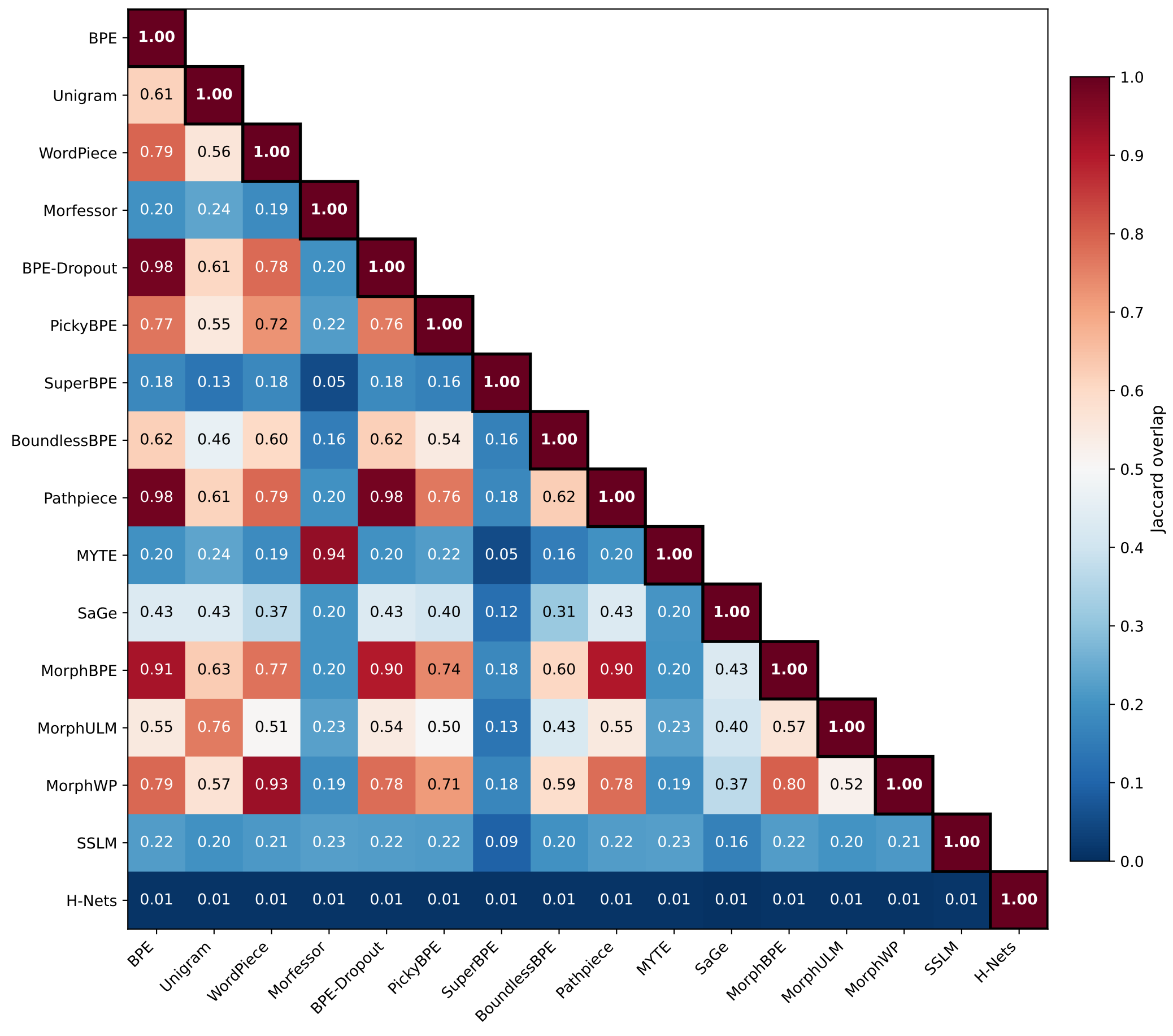
Vocabulary Overlap – Arabic (Script, 2 langs)
