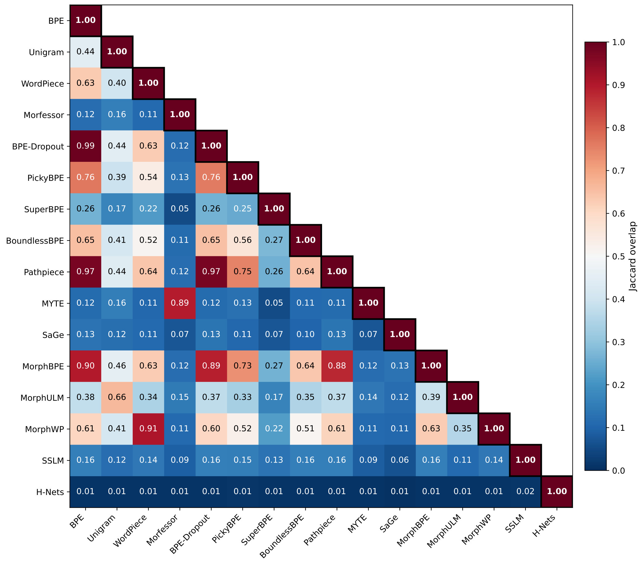
Vocabulary Overlap — Cyrillic (Script, 3 langs)
