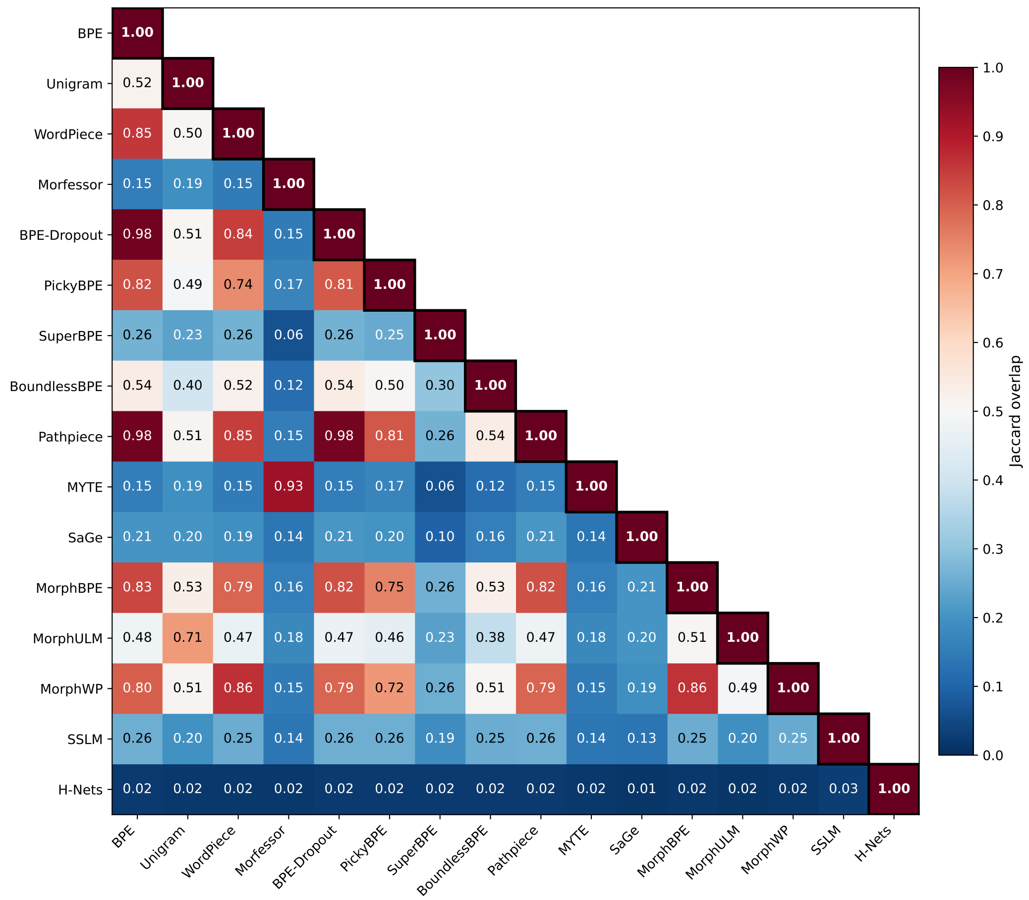
Vocabulary Overlap — Devanagari (Script, 2 langs)
