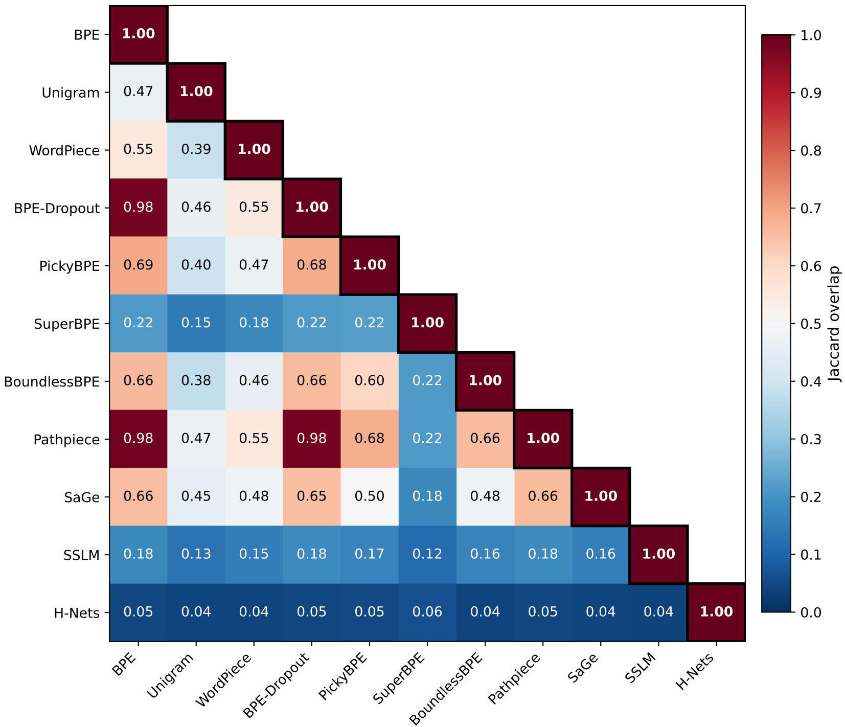
Vocabulary Overlap — eng
