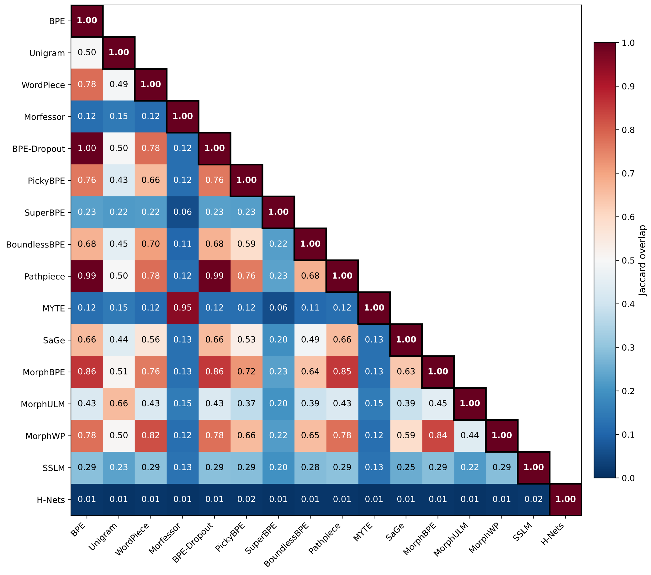
Vocabulary Overlap — heb
