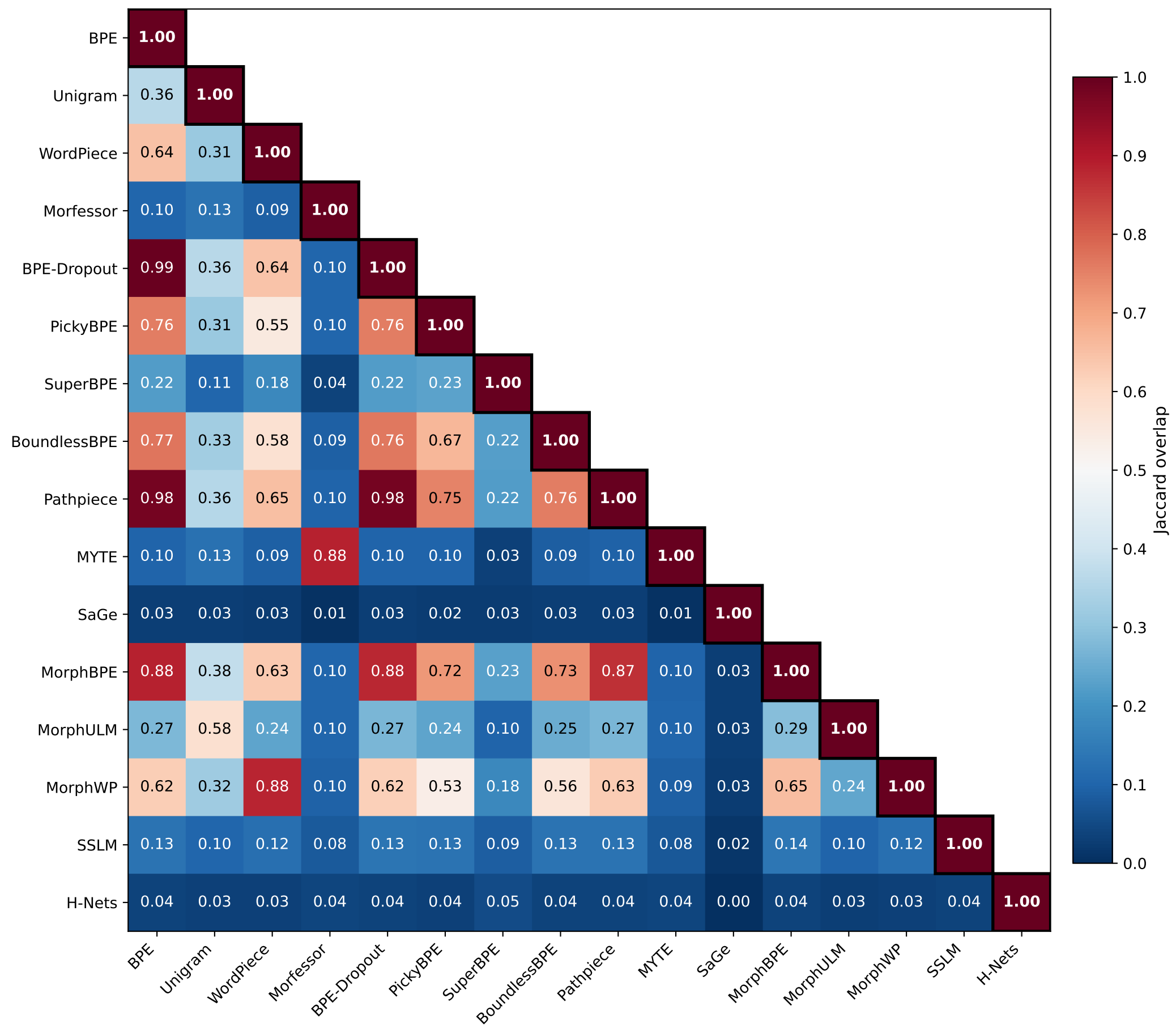
Vocabulary Overlap — hrv
