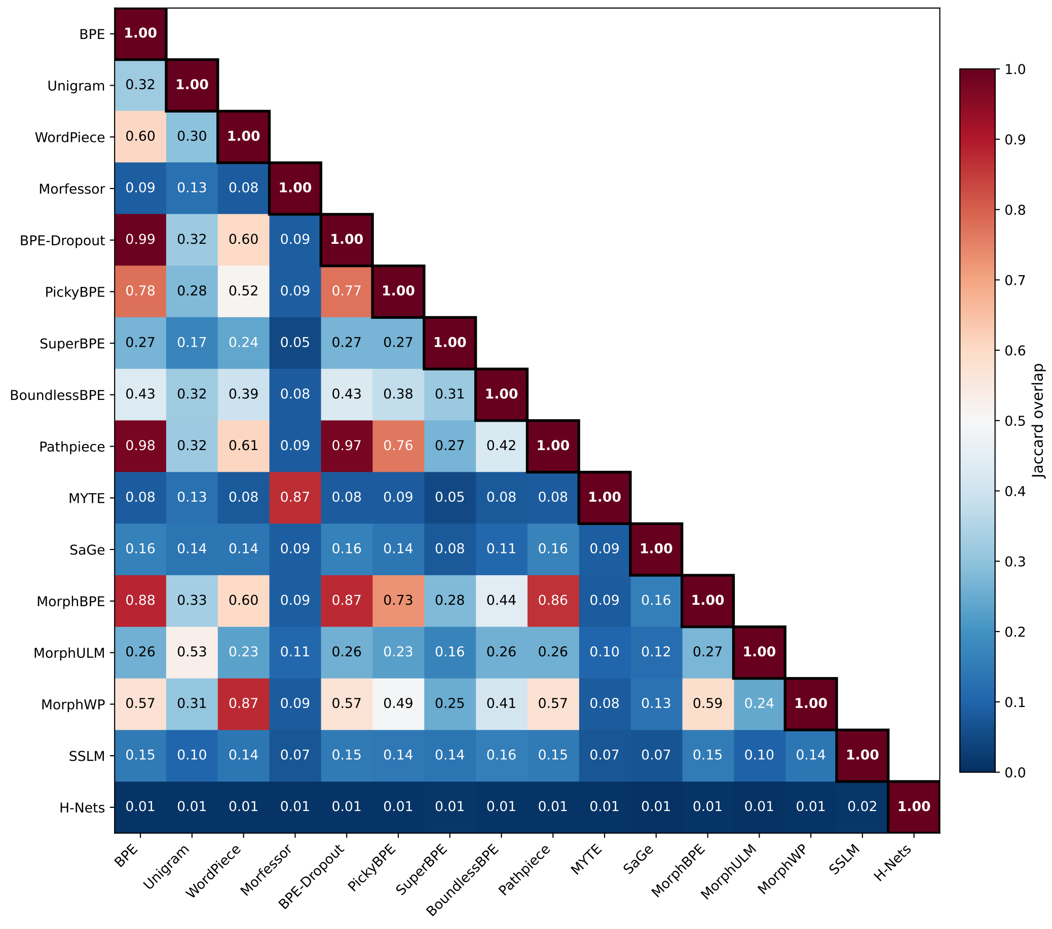
Vocabulary Overlap — rus
