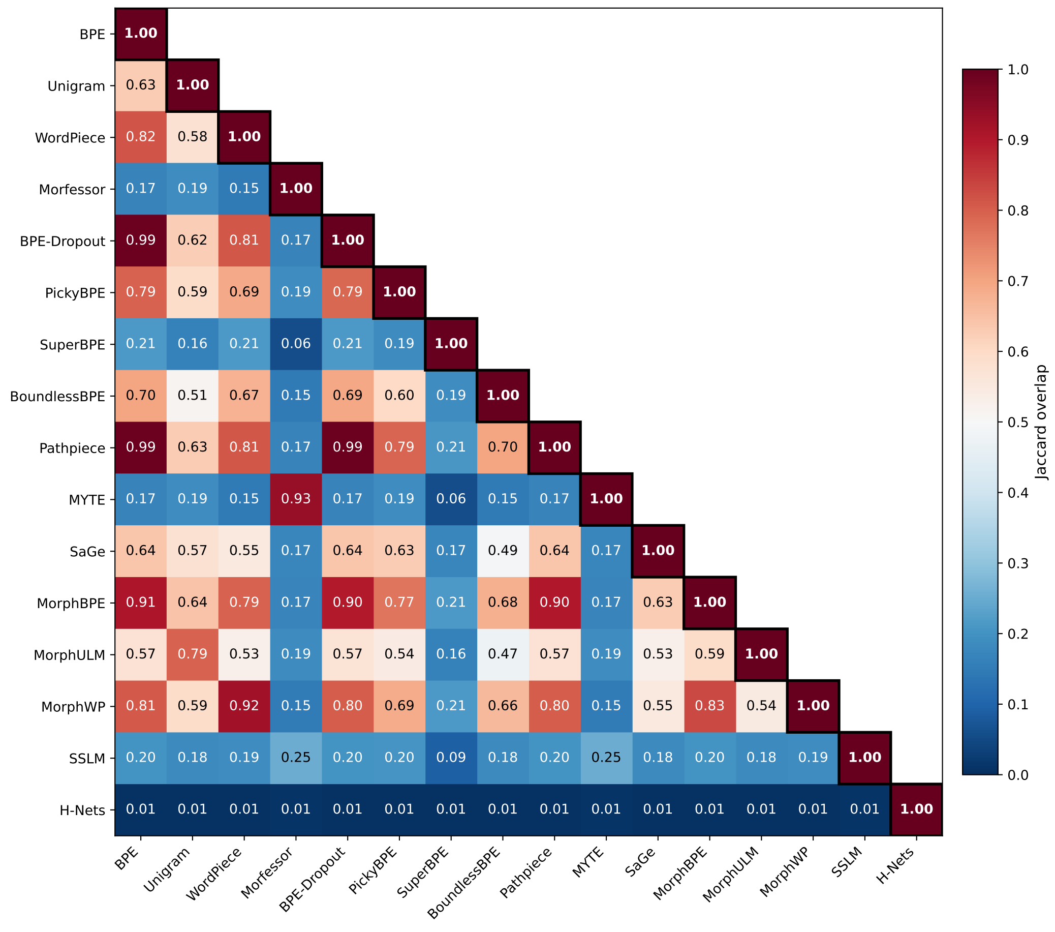
Vocabulary Overlap — snd
