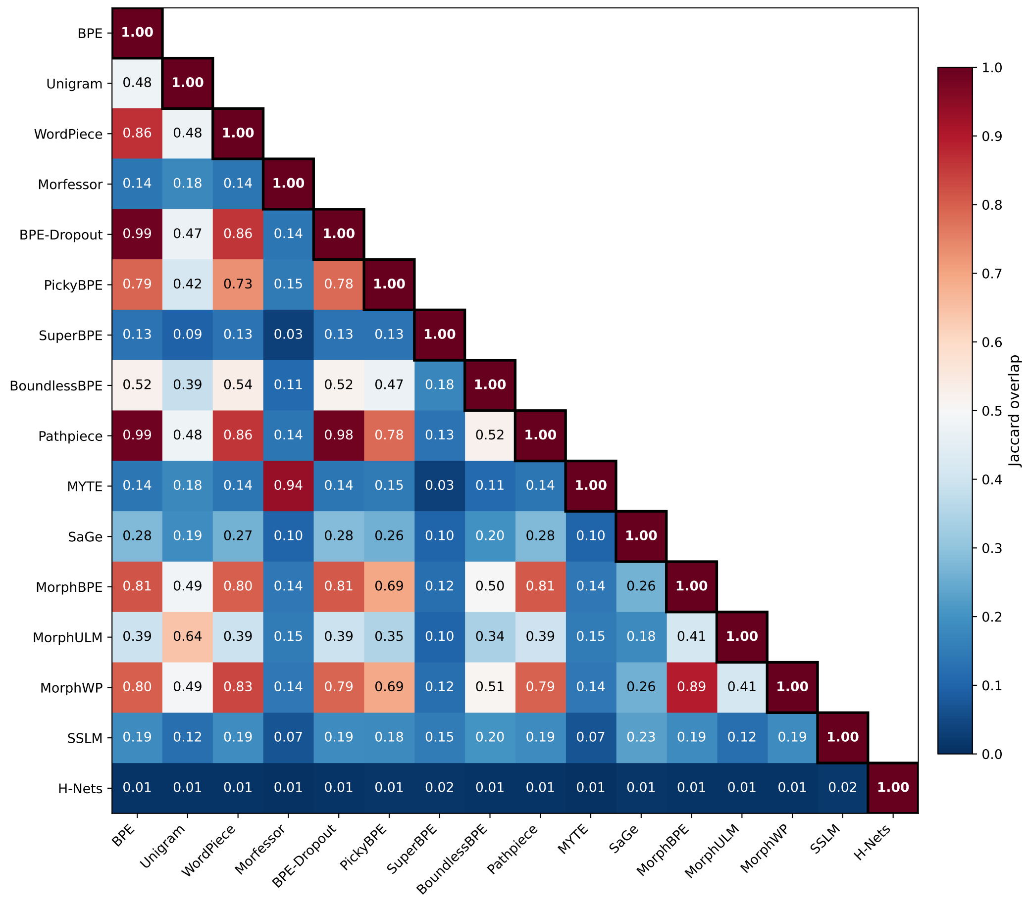
Vocabulary Overlap – tam
