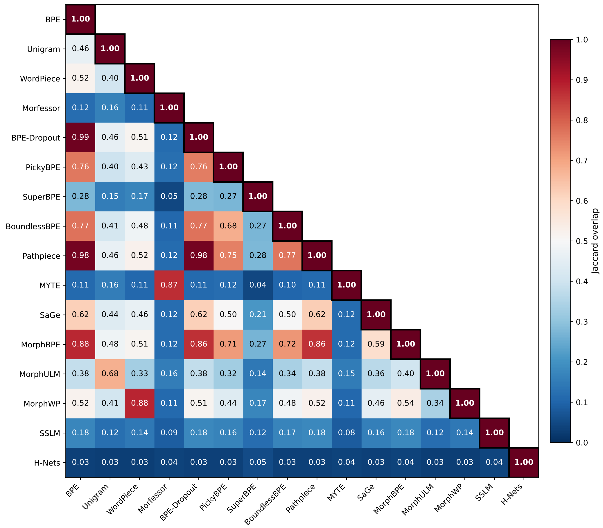
Vocabulary Overlap — tur
