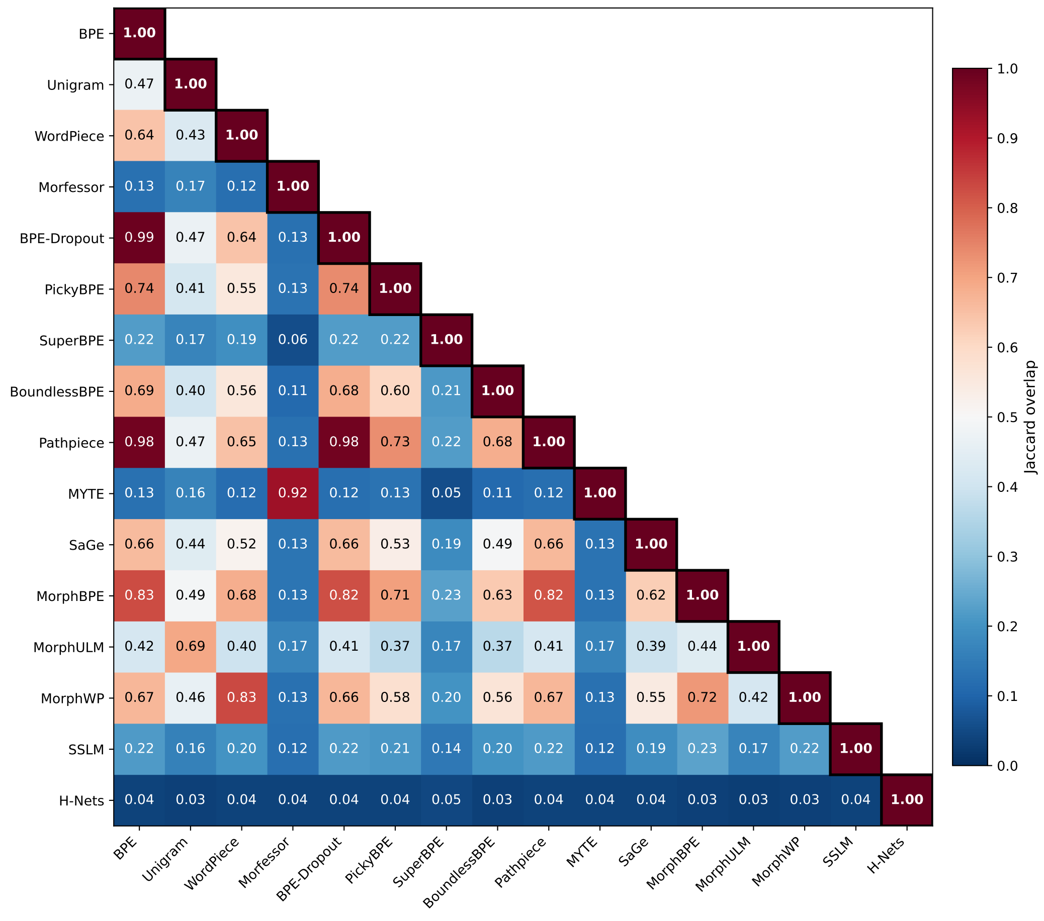
Vocabulary Overlap — Analytic &amp; Introfleixive (Typology, 3 langs)
