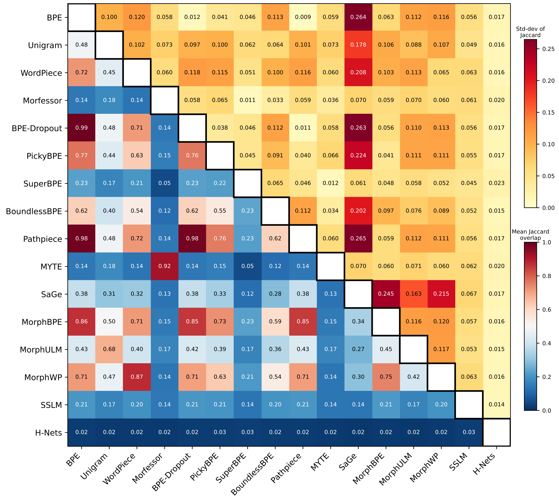
Vocabulary Overlap — Fusional & Analytic (9 langs)
