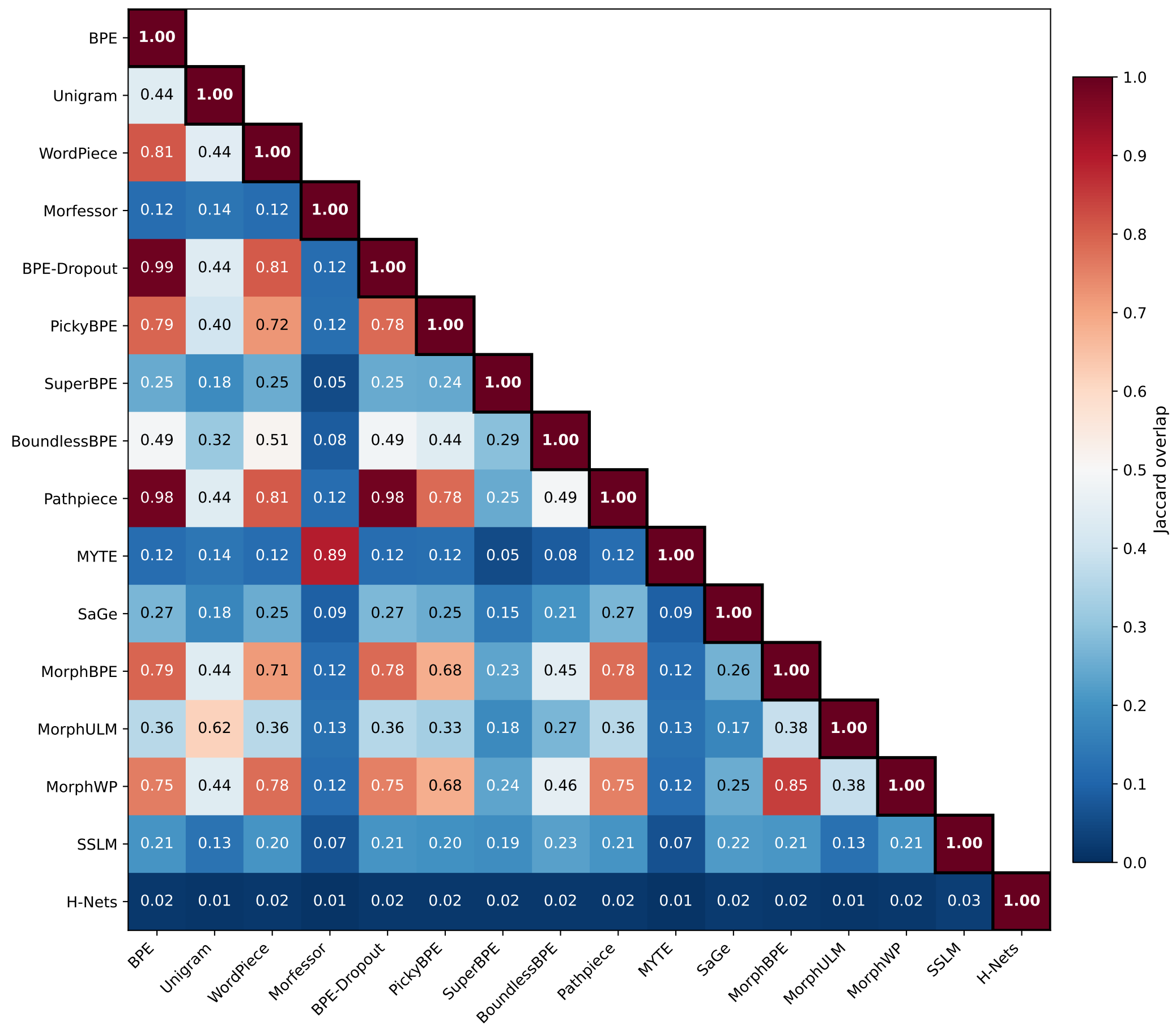
Vocabulary Overlap — Malayalam (Script, 1 lang)
