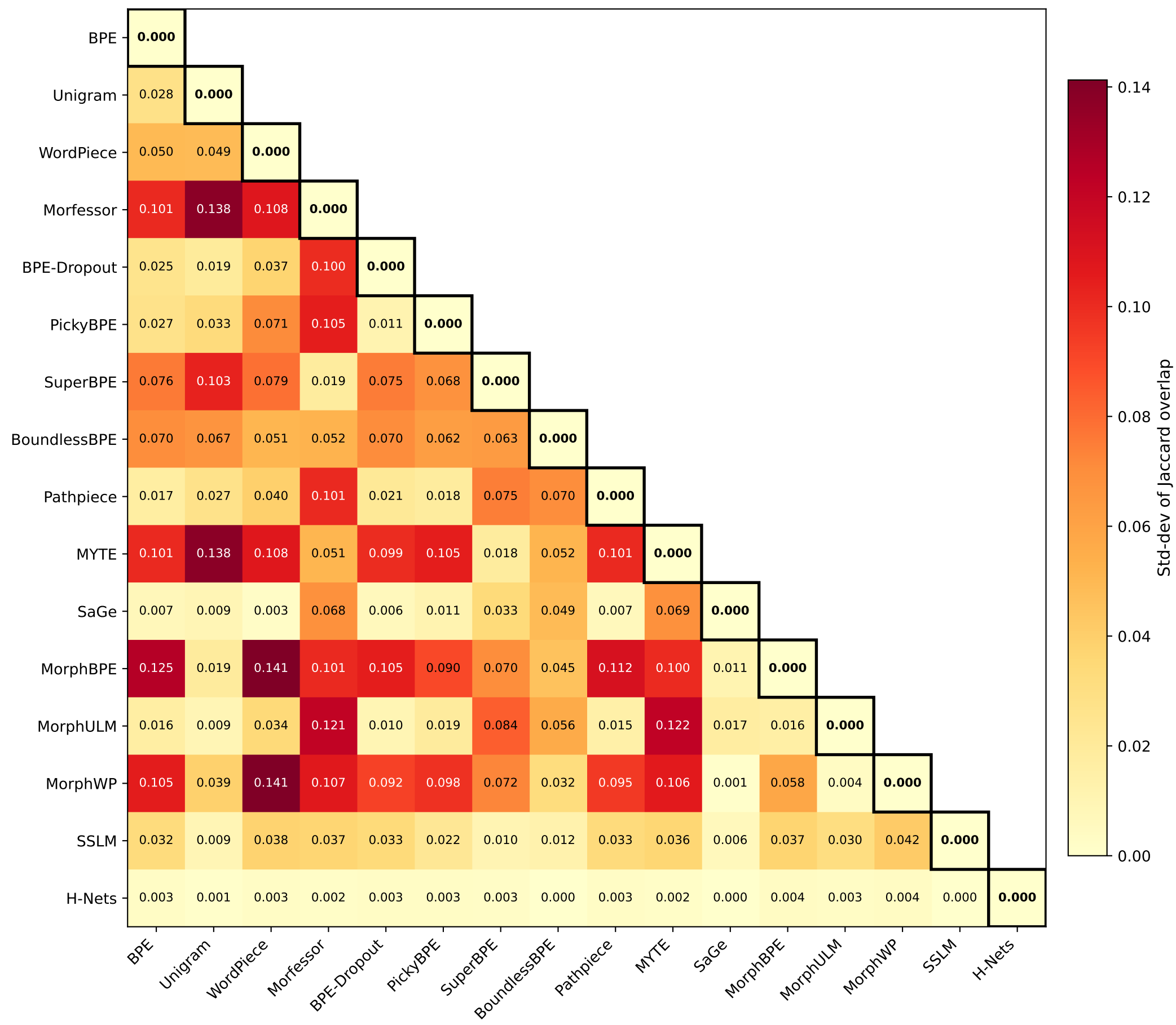
Jaccard Overlap Std-Dev — Devanagari (Script, 2 langs)
