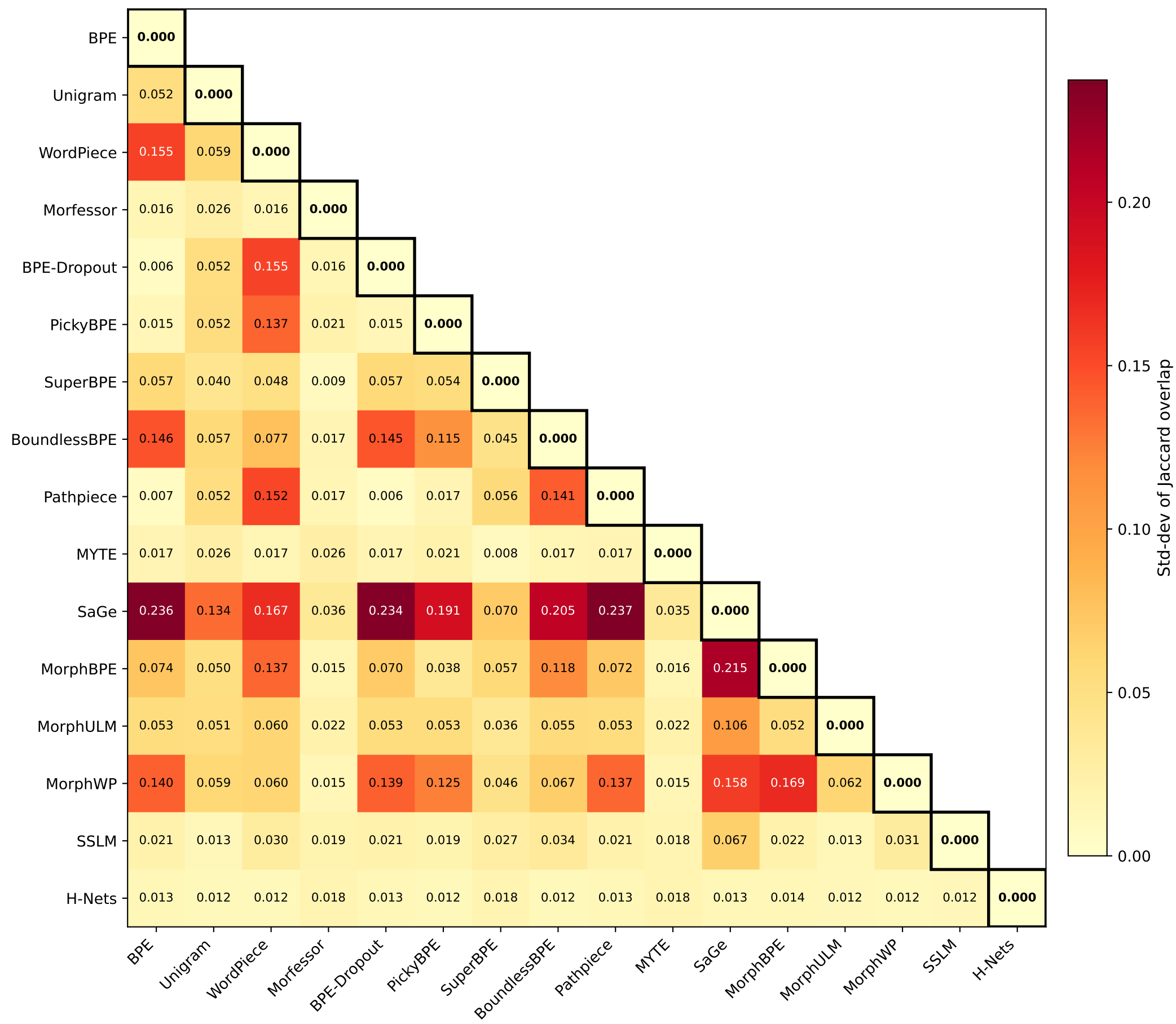
Jaccard Overlap Std-Dev — Agglutinative (Typology, 9 langs)
