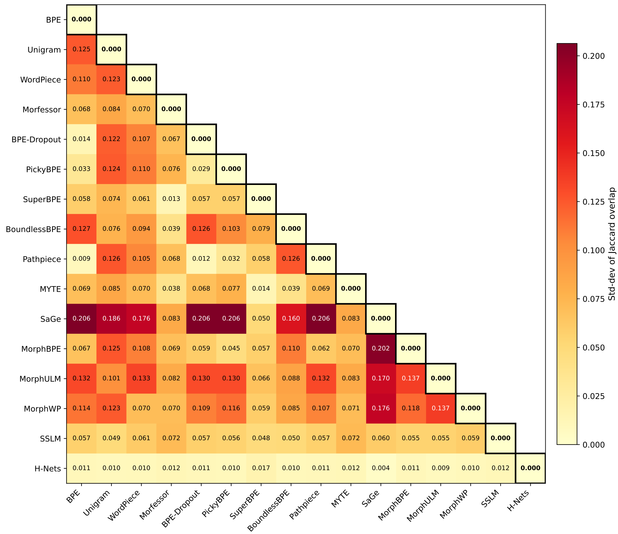
Jaccard Overlap Std-Dev — Fusional (Typology, 6 langs)
