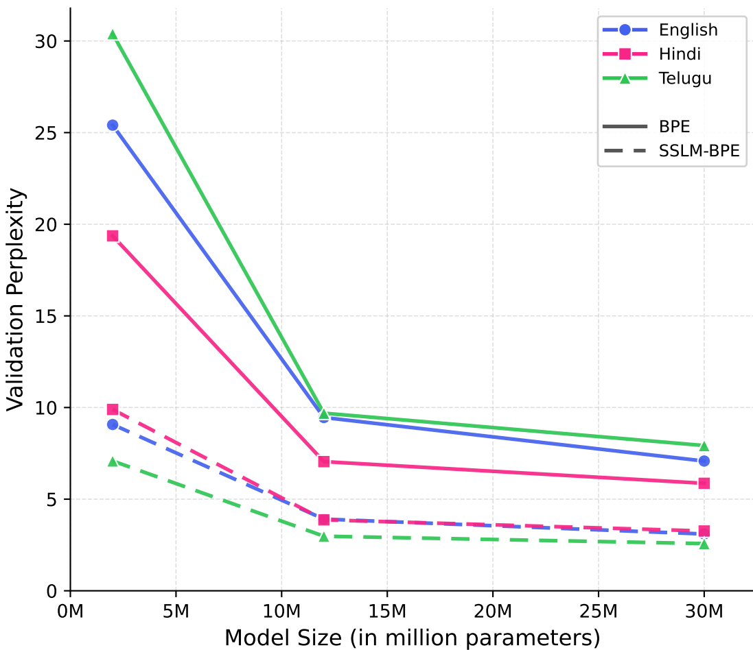
Perplexity vs. Model Size
