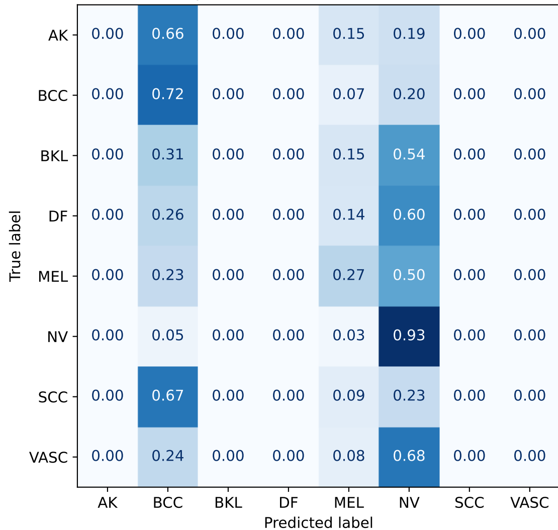
dp: multiclass — Row-normalized
